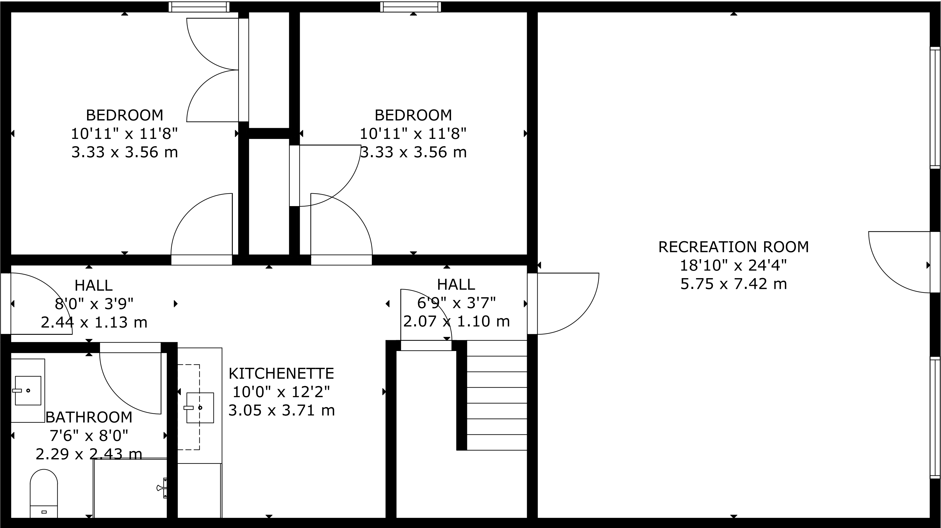
BASEMENT
